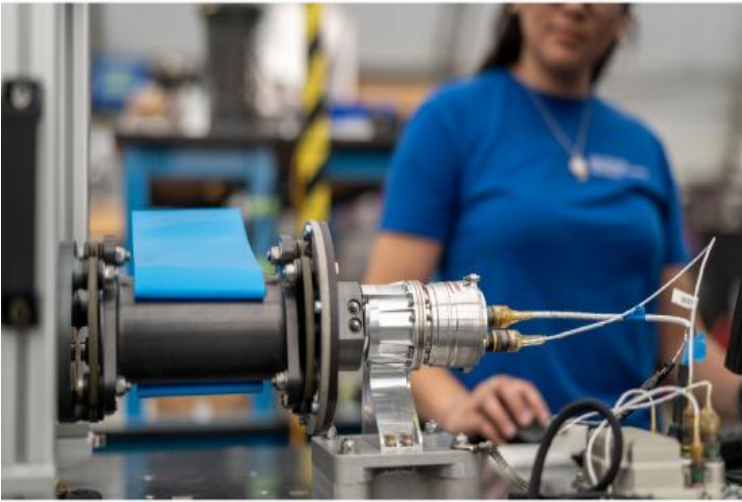
Test engineer Aryssa performing loads testing on our control surface actuators.
